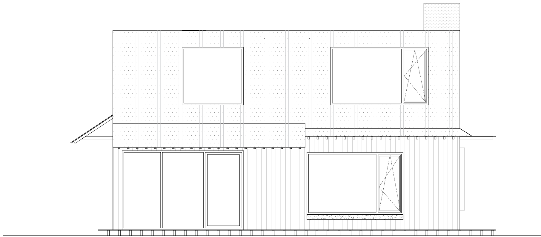
SOUTH FACADE
