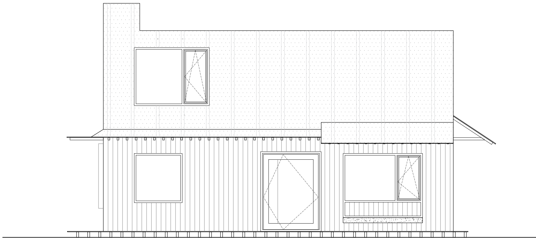
NORTH FACADE
